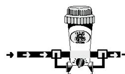
In Ground Off-Line Installation (after heater if installed)
