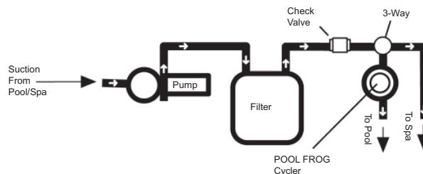
Pool and Spillover Spa Combination
