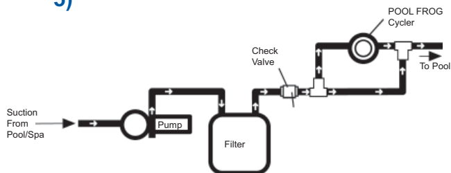
High Flow (over 80 gpm) Installation
